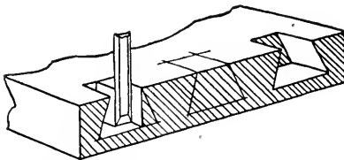
FIG. 433. CHISELING OUT MORTISE.
